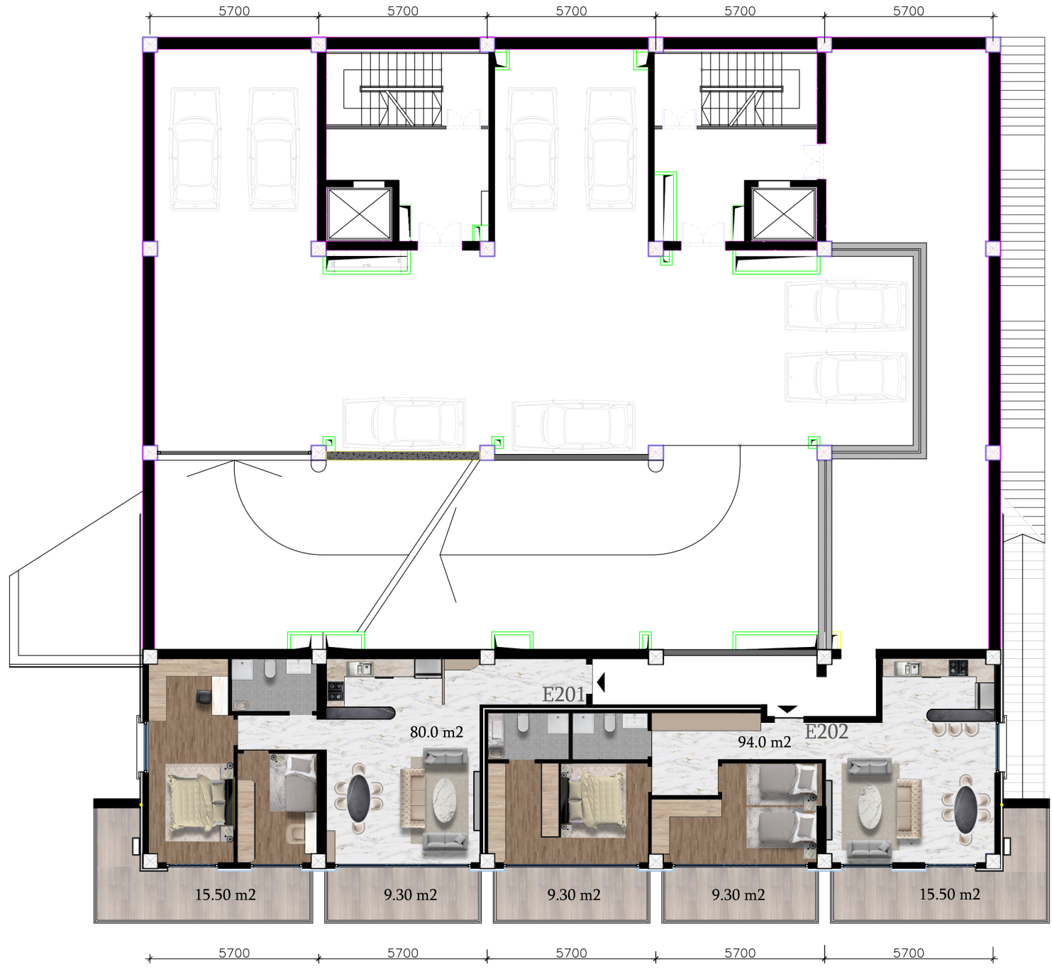
Floorplan at -9.90 m
